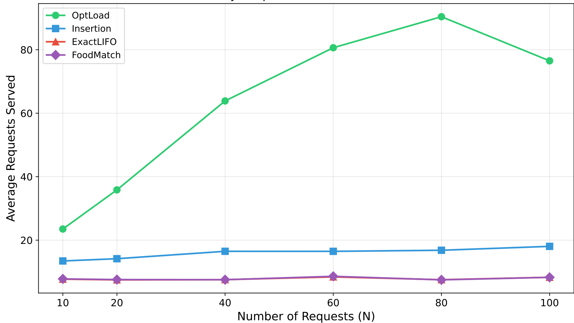
Scalability: Requests Served vs Problem Size
